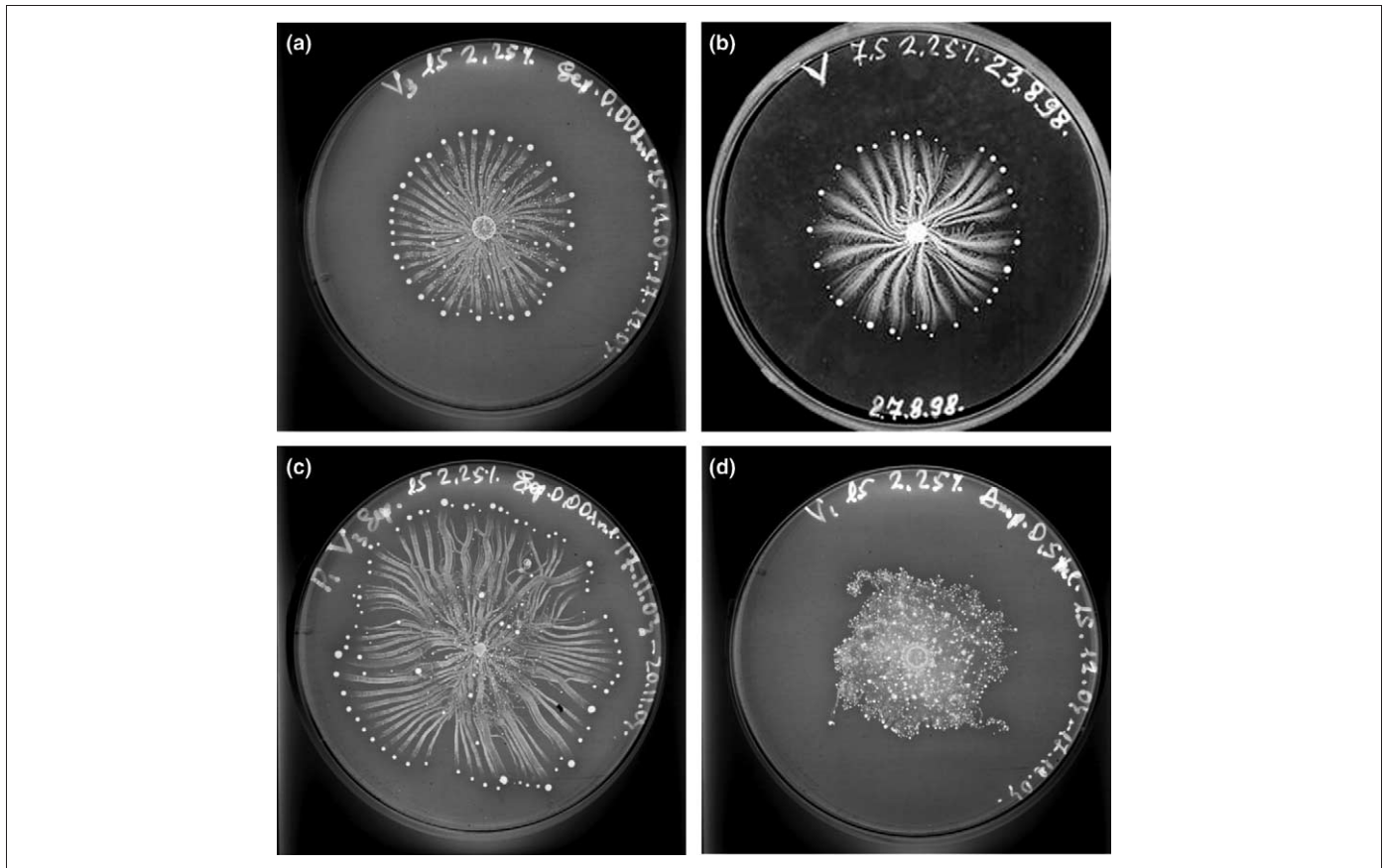
Figure 2. Colonial response to non-lethal stresses. (a) The response of a colony of Paenibacillus vortex to septrin (co-trimoxazole), which inhibits synthesis of folic acid and suppresses cell reproduction, is shown ( 15 \text{ gl}^{-1} peptone and 2.25% agar with added antibiotic). On the basis of comparisons of model simulations with colonial patterns and microscope observations, it was proposed that, in response to septrin, bacteria enhance their cooperation by intensifying chemotactic attraction to form larger vortices; they also elevate repulsive chemotactic responses to signals emitted by the bacteria behind the vortices, which helps push the large vortices faster away from the stress they detect (not 'knowing' that there is antibiotic ahead as well) [9,40]. (b) Colonial development under metabolic stress due to nutrient deficiency is shown – no antibiotic, but half the level of nutrients. We emphasize the abundance of small vortices in this case and slower colonial expansion compared with (a). The pictures were taken after (a) 2 days and (b) 4 days of growth. These differences further support the idea of enhanced cooperation in the presence of septrin. (c) Growth was started from a cluster of bacteria taken from a colony grown in the presence of septrin. Comparison of (c) and (a) illustrates colonial memory and 'learning from experience' (growth conditions are the same in both). Memory can be erased by growing the bacteria on substrate with no antibiotic or in LB growth media. (d) Disorganized colonial development in response to ampicillin (which distorts cell wall structure) is shown. It might appear that ampicillin simply impairs communication-based coordination. However, colonial learning from experience can lead, under some conditions, to faster expansion in the presence of ampicillin.
