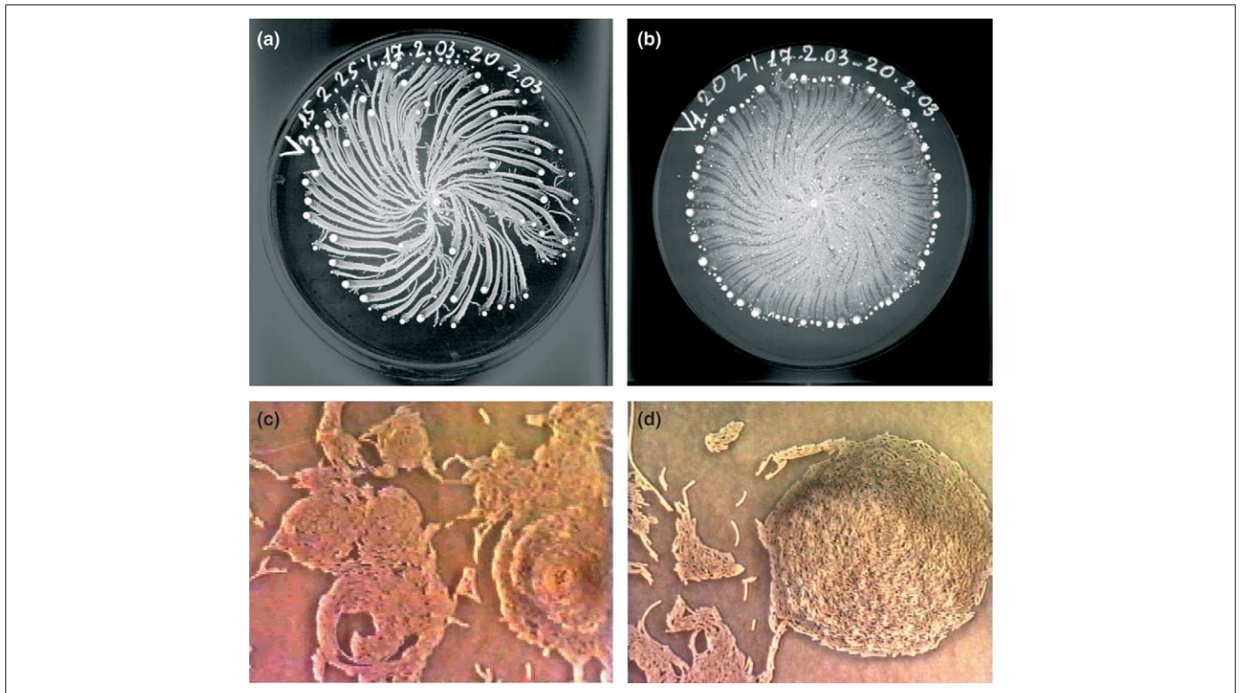
Figure 1. Cooperative hierarchical organization. Complex patterns developed after three-day growth of the Paenibacillus vortex bacteria (taken from the same culture) on 8.8 cm diameter plates, with (a) 15 \text{ gl}^{-1} peptone and 2.25% agar; and (b) 20 \text{ gl}^{-1} peptone and 2.0% agar (the substrate was richer and softer). The bacterial population of these colonies is greater than the human population on earth, however, they coordinate their behavior. Each vortex (bright dot) is composed of many cells that swarm collectively around their common center at \sim 10 \text{ micron sec}^{-1} . The vortices vary in size from tens to millions of bacteria, according to their location in the colony. Both clockwise and anticlockwise rotating vortices are observed, although the majority has the same handedness. The cells in the vortex replicate, and the vortex expands in size and moves outward as a unit, leaving behind a trail (the vortex branch) of motile but usually non-replicating cells. The twist of the vortex branch is determined by the handedness of the vortex rotation. The dynamics of the vortices are quite complicated and include attraction, repulsion, merging and splitting of vortices. However, from this complex, seemingly chaotic movement, a colony with complex but non-arbitrary organization develops, as shown in the top pictures. (c,d) Snapshots from a video recording taken during formation of new vortices are shown (magnification \times 500 , the pictures are \sim 100 microns wide; the rods are the individual bacteria). (c) The dynamics of vortex formation within the branch are shown; an embryonic vortex, similar to the one on the right side of (c), organizes its structure, grows and consequently leaves the branch – as occurs in (d).
