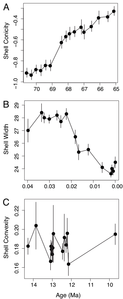
Fig. 1. Examples of fossil trait sequences that are best fit by each of the three evolutionary models. (A) Directional evolution: shell shape in the planktonic foraminifera Contusotruncana from DSDP site 384 (45). (B) Unbiased random walk: shell width in the land snail Mandarina (46). (C) Stasis: shell shape (convexity) in the bivalve Chesapecten nefrens (34).
